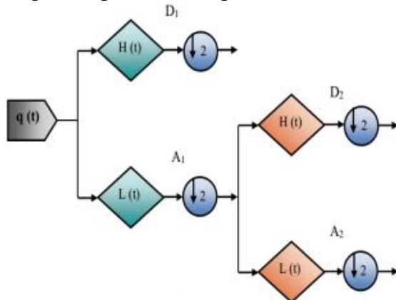
Figure 2: DWT decomposition
