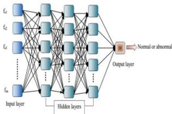
Figure 3: DNN structure
