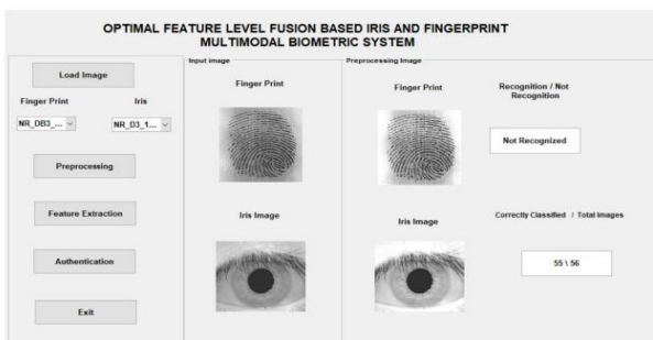
Figure 8: GUI Representation
