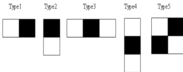
Figure3: Haar features in viola-Jones.
