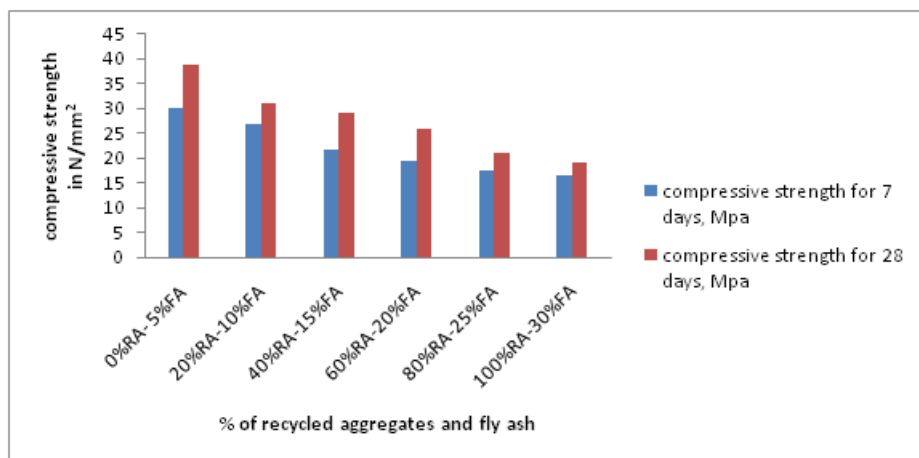
Fig 5: compressive strength of concrete with fly ash
