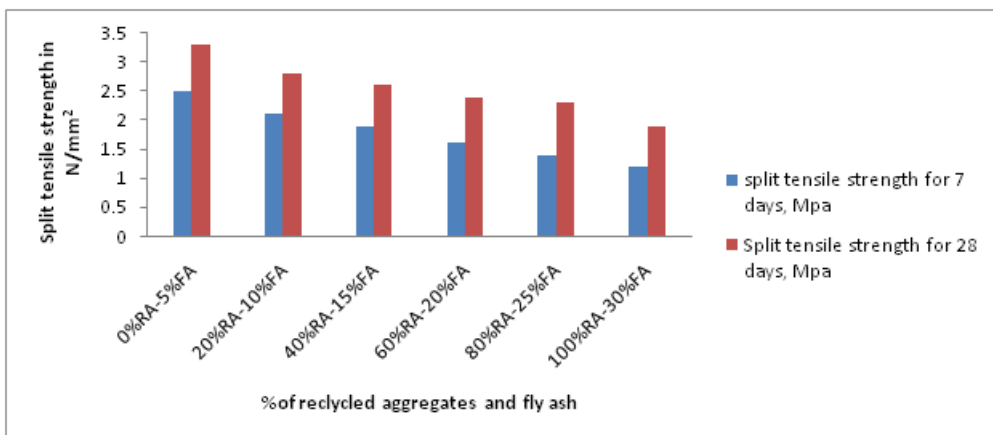
Fig 6: Split tensile strength of concrete with fly ash
