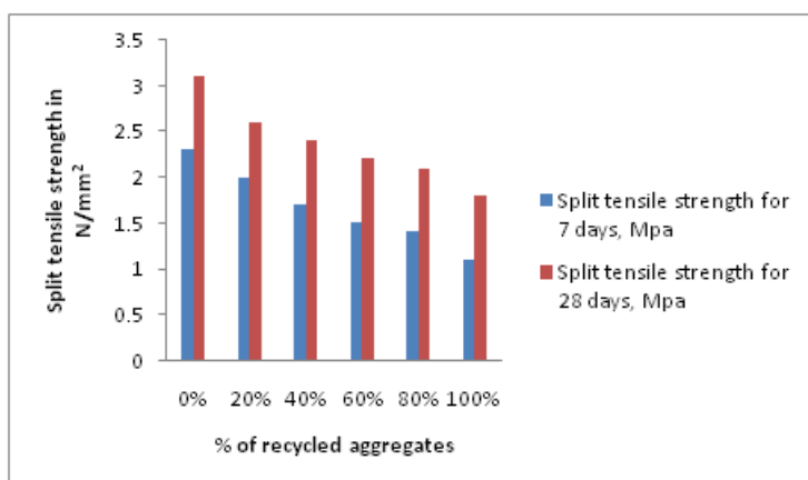
Fig 4: split tensile strength of concrete
