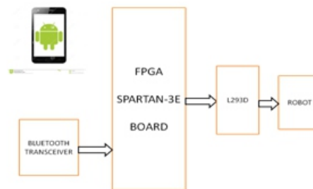
Figure1: Block diagram
