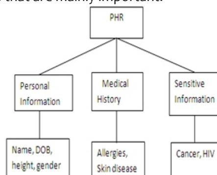
Fig 1. The attribute
