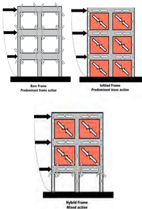
Fig 1.2 Behaviour of load transfer in buildings with infills Infill walls influence the behaviour of a RC frame: (a) a bare frame; (b) infill walls must be uniformly distributed in the building; and (c) if the infills are absent at the ground floor level this modifies the load path, which detrimental to earthquake performance.
