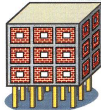
Fig 1.1 Typical example of first soft storey
