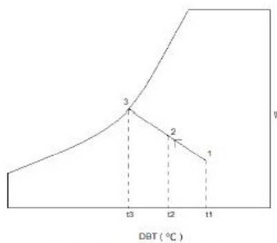
Fig.1 Cooling and humidification process
