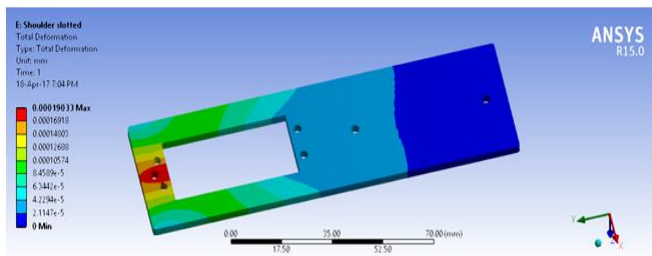
Shoulder Analysis (Total Deformation)
