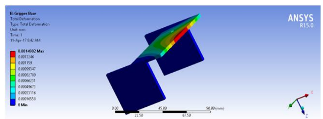
Gripper Analysis (Total Deformation)
