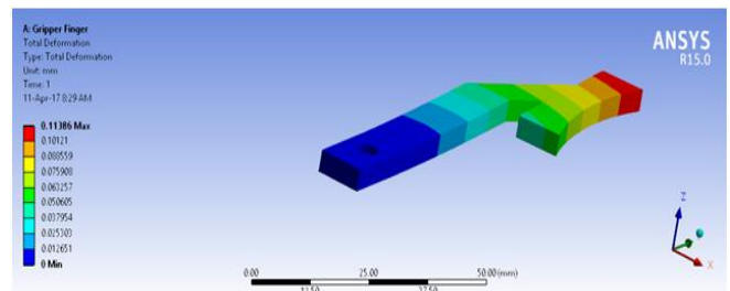
Grippers Analysis (Total Deformation)
