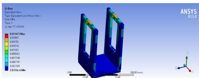
Base Analysis (Equivalent Stress)
