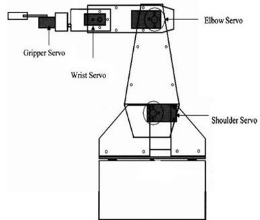
Figure 1: Design Overview of Robotic Arm.
