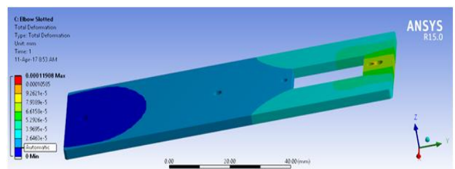
Elbow Analysis (Total Deformation)
