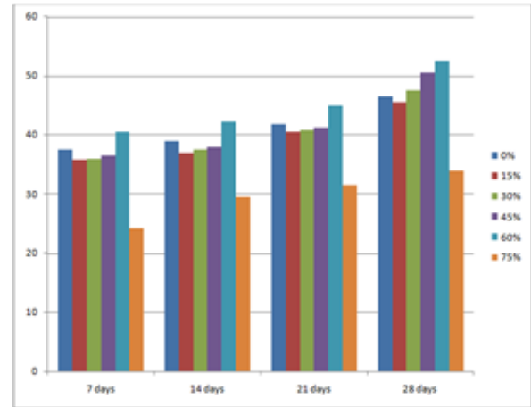
Fig 3.0: Showing the Curing days against Compressive Strength.
