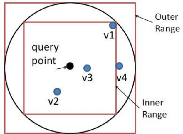
Fig. 2. Illustration for kNN-R Algorithm when k = 3.
