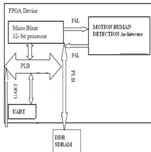
Fig 3 System Overview
