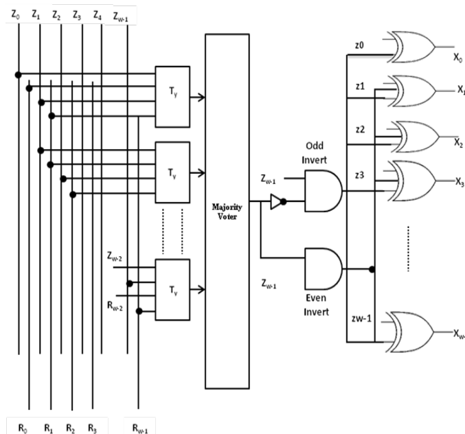
Fig.7. Decoder Architecture Scheme 3.
