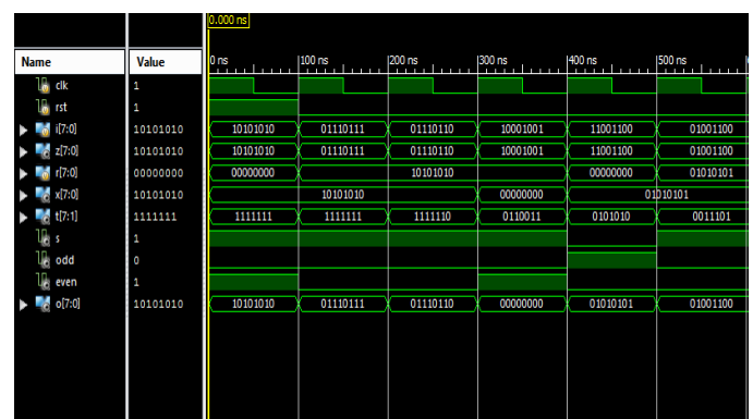
Fig.11. Scheme 3 Decoder
