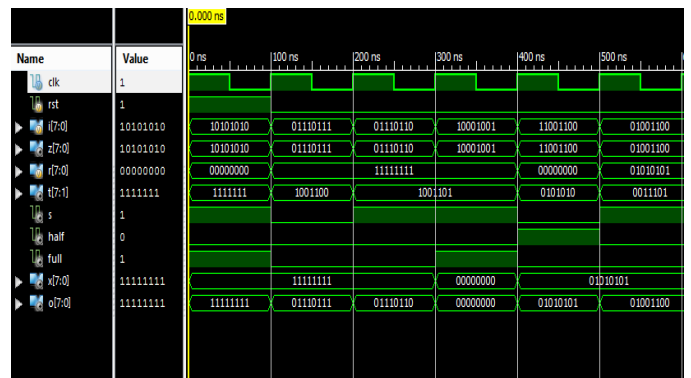
Fig.10. Scheme 2 Decoder.
