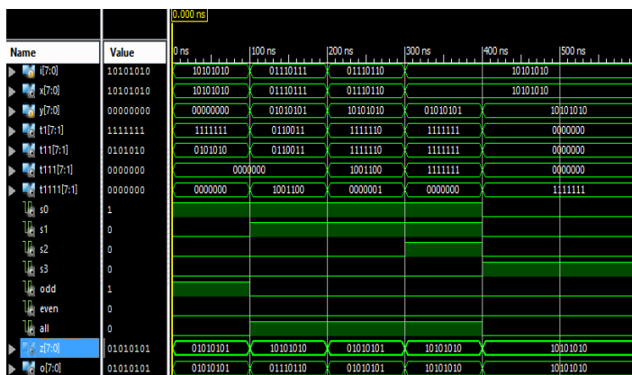
Encoder Scheme 3
