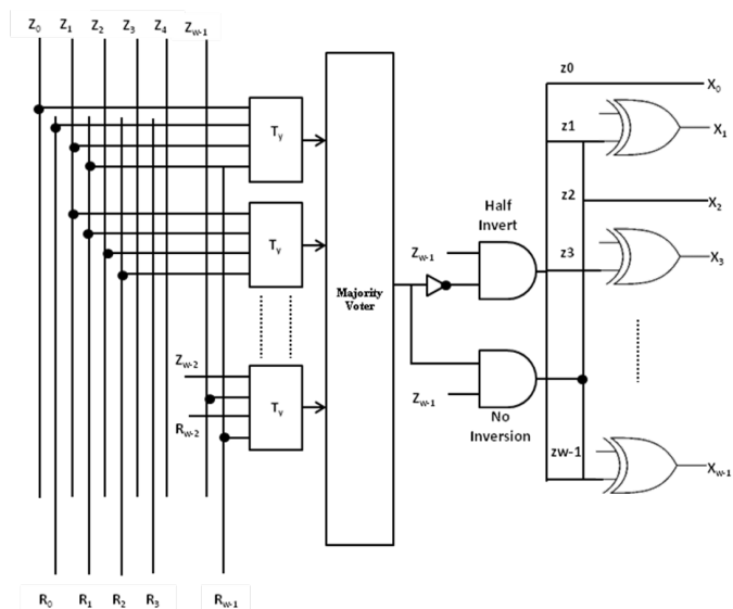
Fig.5. Decoder Architecture Scheme 1.
