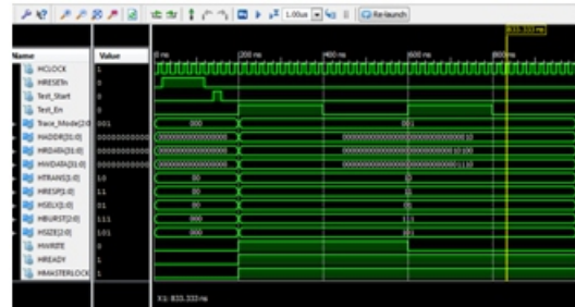
Fig-6: AHB Lite tracer input outputs with different modes
