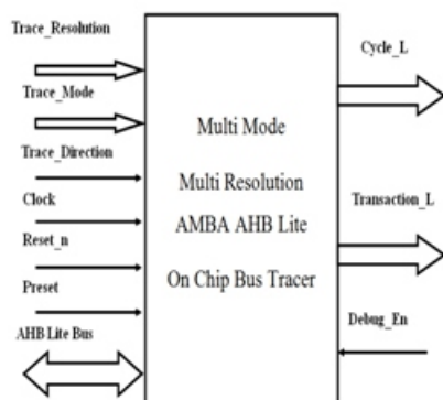
Fig-2: Multi mode multiresolution AHB Lite Tracer
