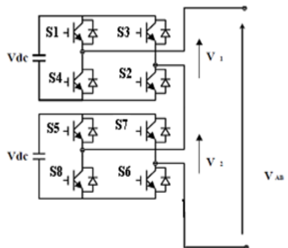
Fig 1. Five level cascaded H-bridge multilevel inverter
