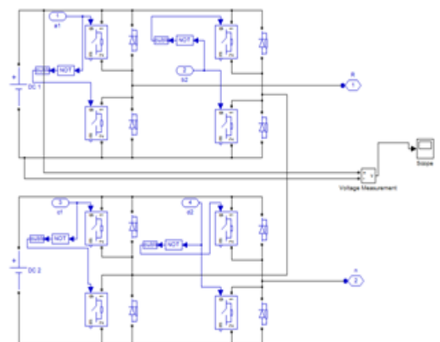
Fig.13. Cascaded H-bridge circuit
