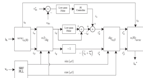
Figure 4: dq-based current reference generator block diagram .
