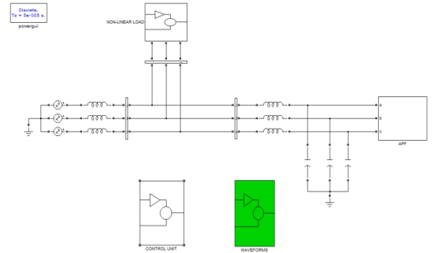
Fig.5 Simulation Circuit
