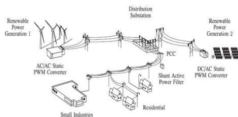
Fig. 1. Stand-alone hybrid power generation system with a shunt active power filter.
