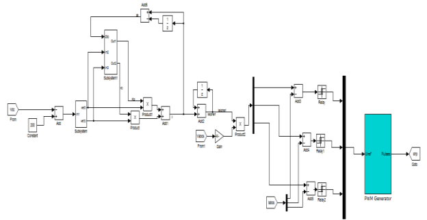
Fig.6 CONTROL UNIT
