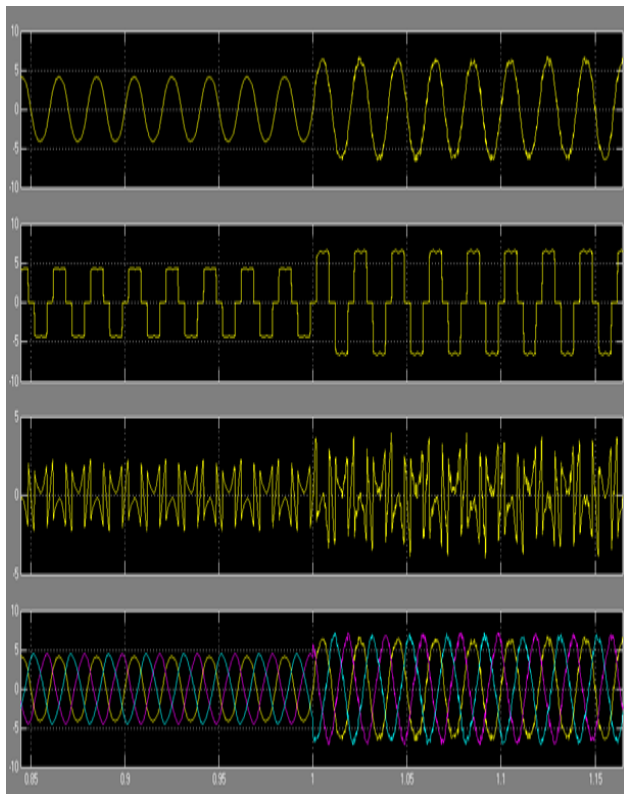
Fig.8 ISa,ILa,Iinv,ISabc(zoomed waveforms)
