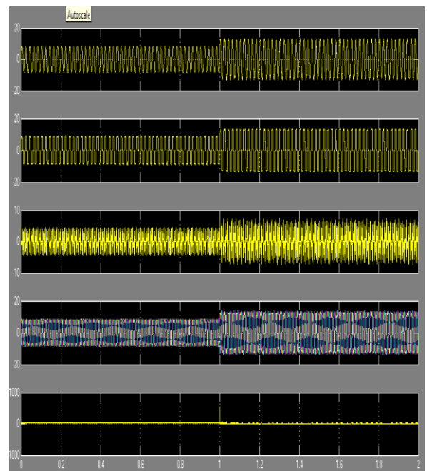
Fig.7 ISa,ILa,Iinv,ISabc,Vdc
