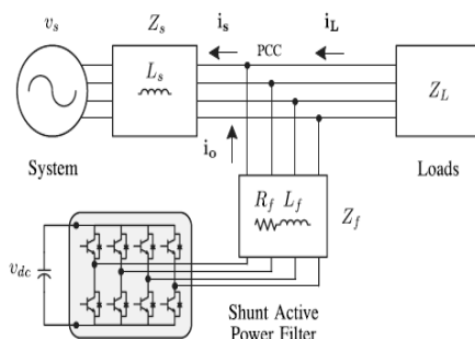
Fig. 1. Stand-alone hybrid power generation system with a shunt active power filter.
