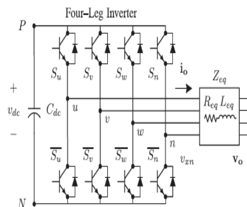
Fig. 3. Two-level four-leg PWM-VSI topology.
