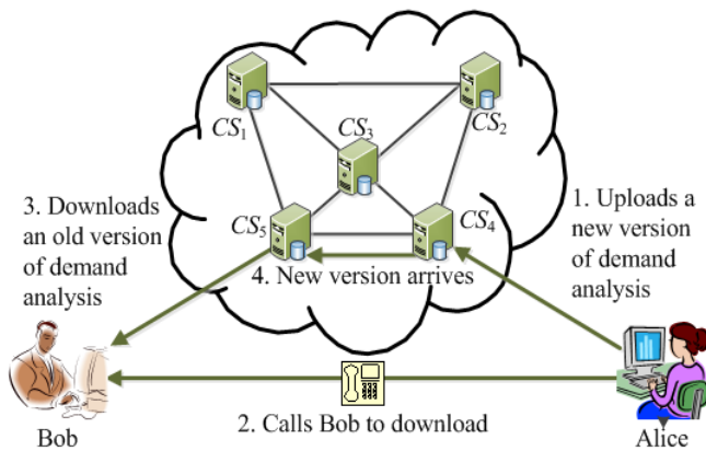
Fig. 1. An application that requires causal consistency
