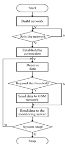
Figure 2. ZigBee master program flow monitoring
