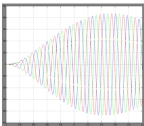
Fig 15: grid voltage
