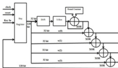
Fig. 4. Architecture of Key Generation Module
