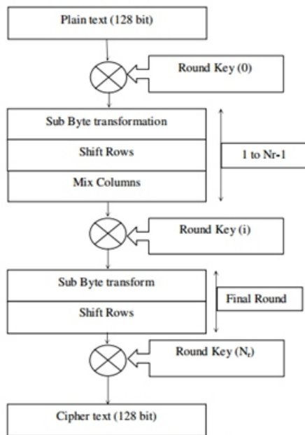
Fig. 1. Algorithm for AES Encryption [2]
