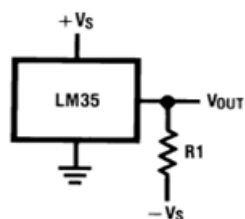
Figure-3: LM35 sensor
