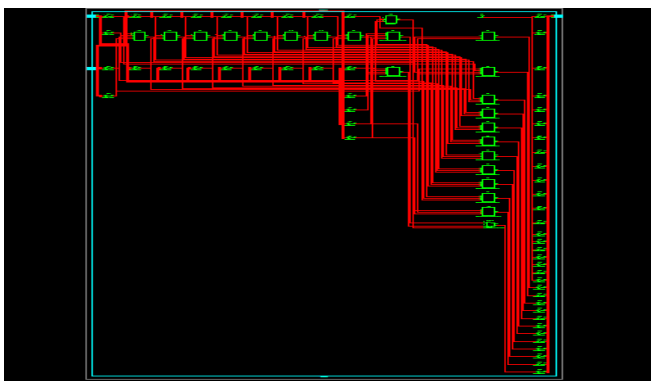
Fig 7. Sub Technology schematic of 32bit error-tolerant adder (ETA)
