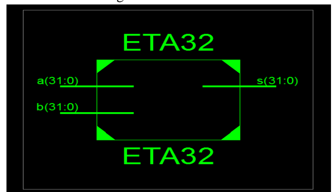
Fig 4. RTL schematic of 32bit error-tolerant adder (ETA)
