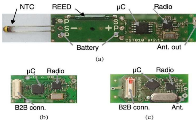
Fig. 5. PCB of sensor nodes for environmental monitoring: (a) for in situ wild-fire detection, (b) for mostly analog, and (c) for mostly digital applications scale .
