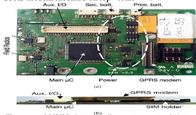
Fig. 7. PCB of the gateway node for environmental monitoring: (a) top view and (b) side view with the GPRS modem mounted on top scale
