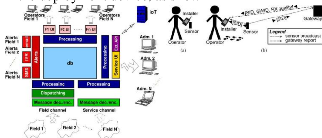
Fig. 10. Application server interfaces.
