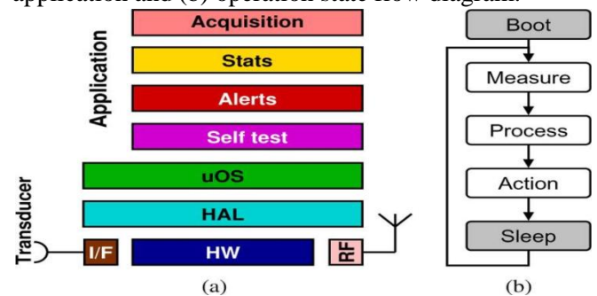
Fig. 6. Sensor node: (a) firmware structure for reference application and (b) operation state flow diagram.
