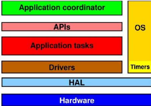
Fig. 8. Gateway firmware block diagram.
