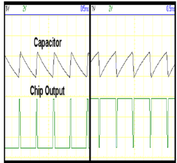
Fig: Trace of a saw tooth charge-discharge cycle of a capacitor and the variable-width PWM square wave output using oscilloscope.
