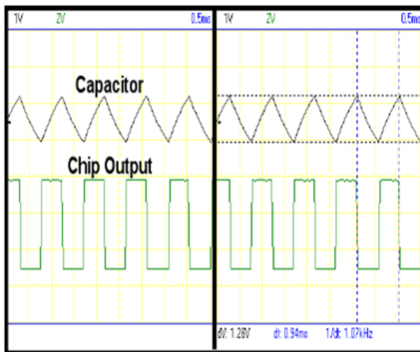
Fig: Oscilloscope graph of a triangular charging –discharging cycle of a capacitor and the square waveform output
