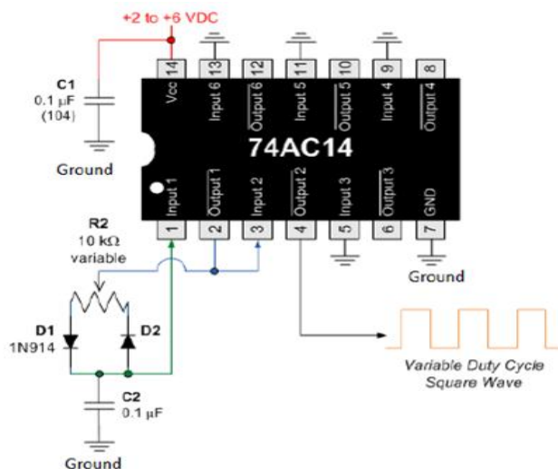
Fig :Pin diagram of changing duty cycle PWM circuit using 74AC14 inverter logic chip
