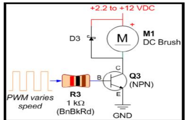
Fig :Circuit Diagram of a pulse-width modulator (PWM)
