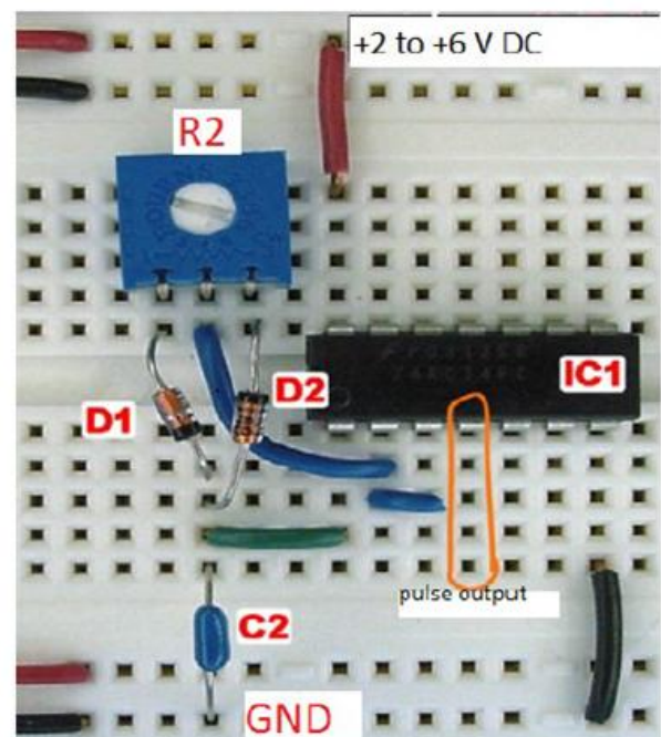
Fig : changing duty-cycle pulse-width modulation circuit board implemented on a breadboard.
