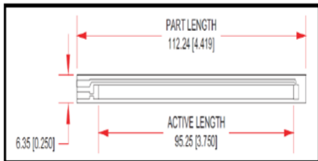
Fig :Dimensional diagram of flex sensor
