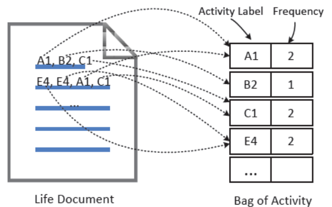
Fig 2: Bag of Activity
