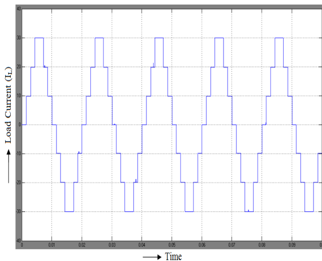
Fig 5.4 Seven levels of Inverter output current ( I_{inv} )
