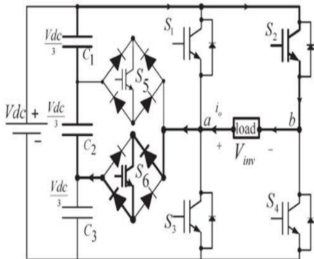
Fig 3.6 Inverter circuit for the output voltage ( -2V_{dc}/3 )
