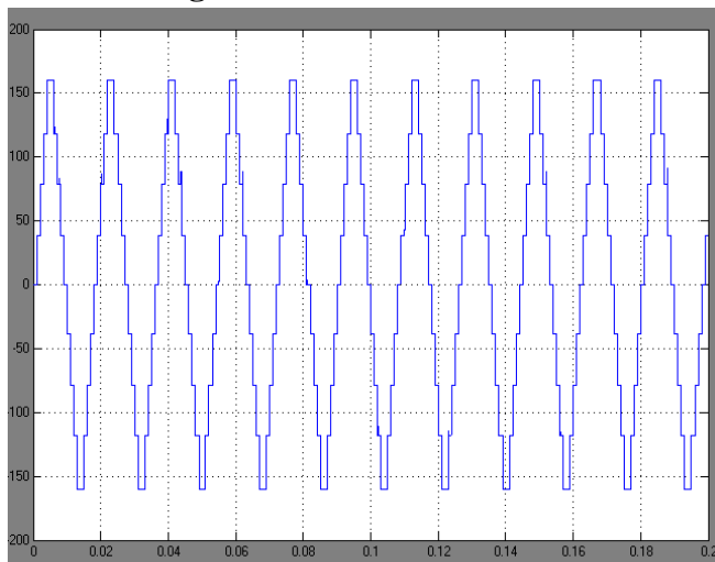
Fig 5.8 Nine level inverter output voltage
