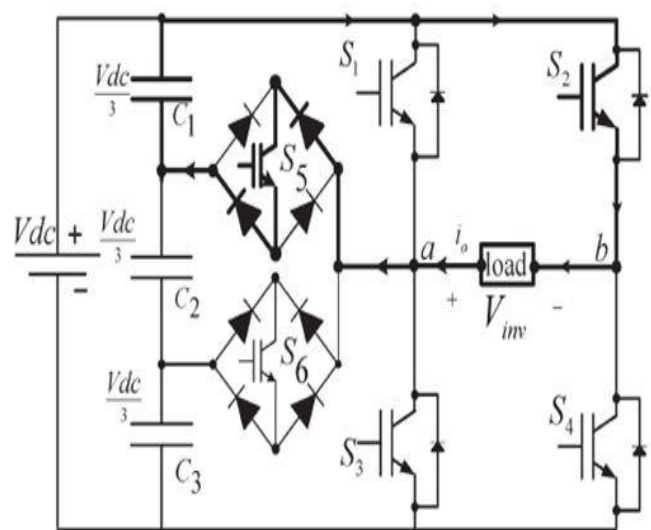
Fig 3.5 Inverter circuit for the output voltage ( -V_{dc}/3 )
