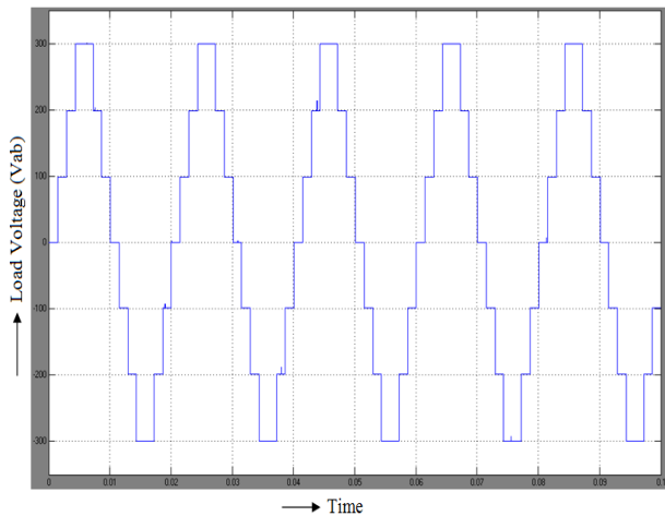
Fig 5.2 Seven levels of Inverter output voltage ( V_{inv} )
