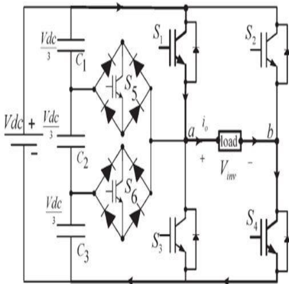
Fig 3.1 Inverter circuit for the output voltage ( V_{dc} )
