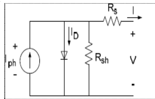
Fig 2.2: PV cell equivalent circuit
