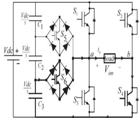
Fig 3.3 Inverter circuit for the output voltage ( V_{dc}/3 )
