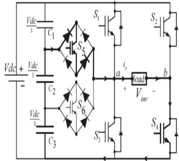
Fig 3.2 Inverter circuit for the output voltage ( 2V_{dc}/3 )
