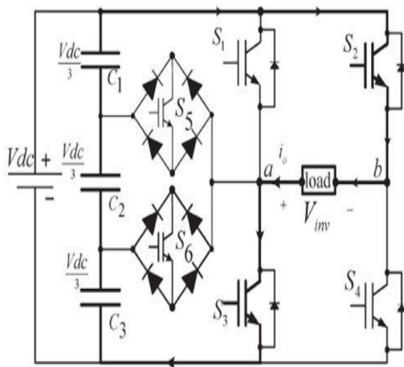
Fig 3.8 Inverter circuit for the output voltage ( -V_{dc} )
