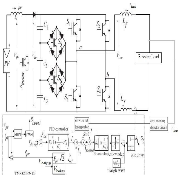
Figure 1.1: Seven-level inverter with closed-loop control algorithm
