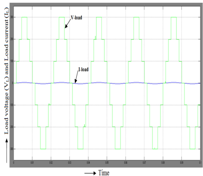
Fig 5.6 Load voltage ( V_{Load} ) and Load current ( I_{Load} ) that are in phase
