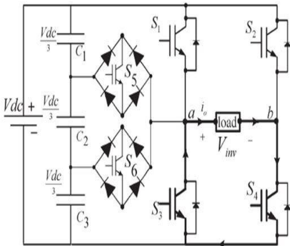
Fig 3.4 Inverter circuit for the output voltage (zero 0)
