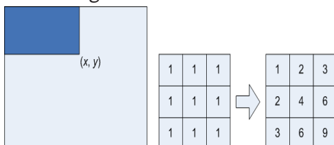
Fig 2. Integral Image Generation. The Shaded Region Represents The Sum Of The Pixels Up To Position (X, Y) Of The Image. It Shows A 3x3 Image and Its Integral Image Representation.
