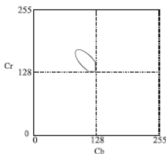
Fig 6. Region Bounding the Skin-Like Colors on the CbCr Color Space.
