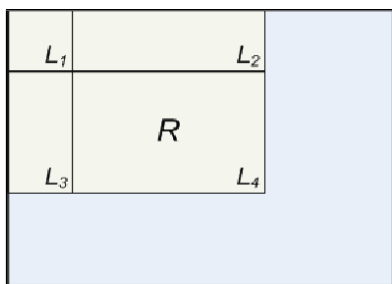
Fig 1. Calculating the area of a rectangle R is done using the corner of the rectangle: L_4 - L_3 - L_2 + L_1 .
