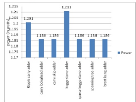
Fig. 14. Power observed in Xilinx
