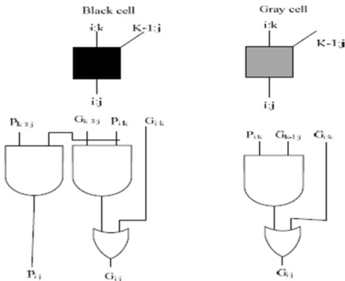
Fig. 3. Black and Gray Cell logic Definitions
