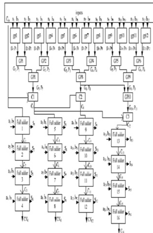
Fig. 5. 16 bit spanning tree adder
