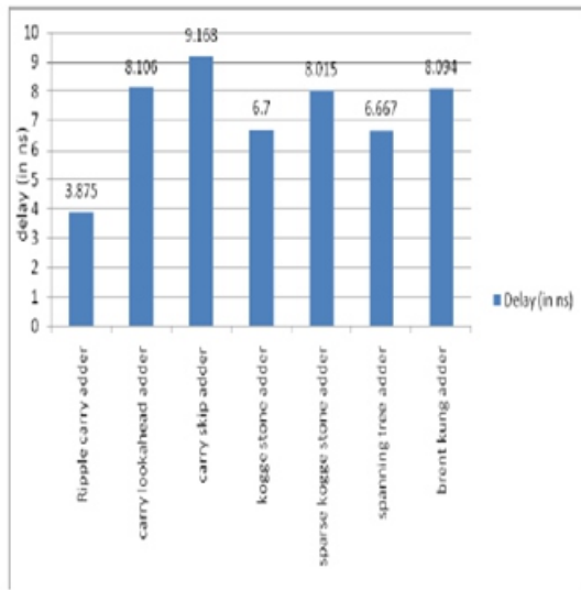
Fig. 11. simulation results for the adder designs
