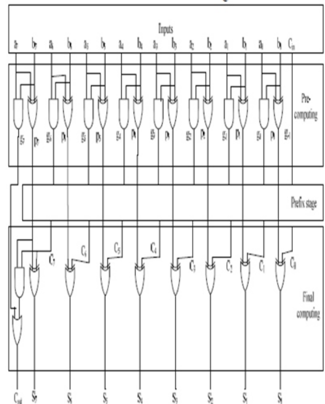
Fig. 2. Parallel-Prefix Structure with carry save notation.
