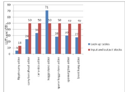
Fig. 13. LUT's and IOB's observed in Xilinx ISE
