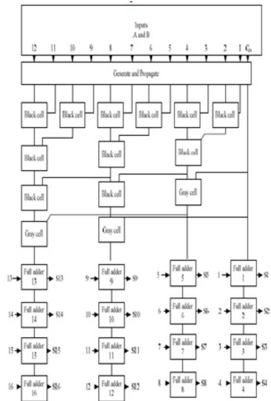
Fig. 4. 16 bit sparse kogge-Stone adder
