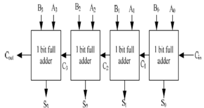
Fig. 1. 4 bit ripple carry adder
