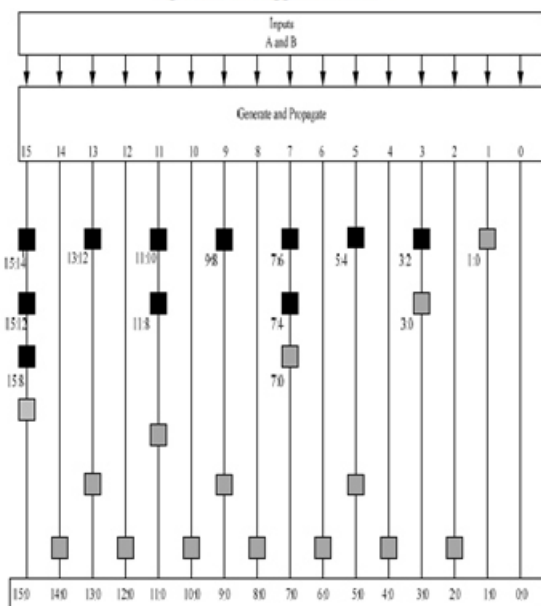
Fig. 7. 16 bit brent kung adder
