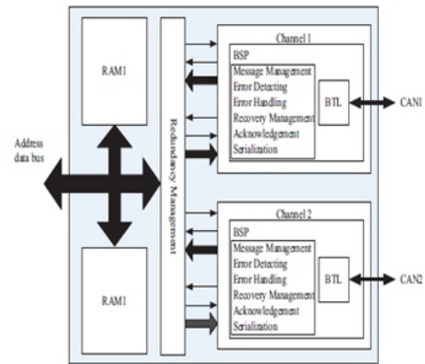
Fig 1. Dual Redundancy CAN-bus Controller Block Diagram.
