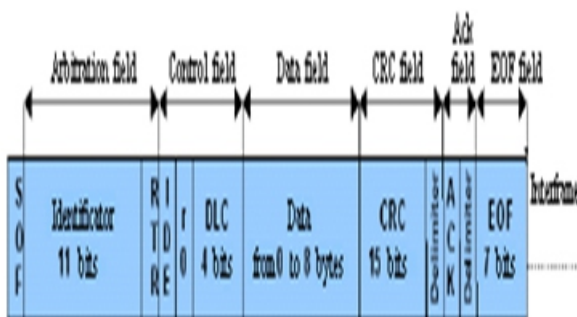
Fig 3: Data Frame Structure
