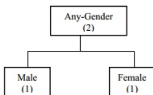
Figure 5. Taxonomy for Gender
