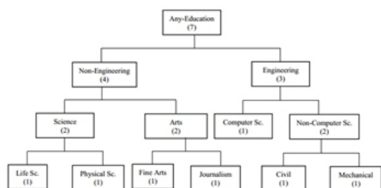
Figure 3. Taxonomy for Education
