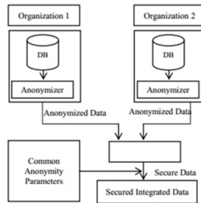
Figure 6. Secure Data Integration
