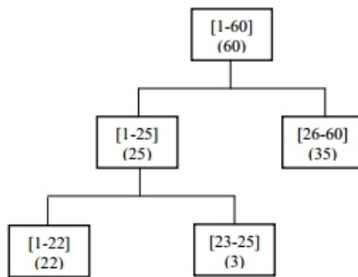
Figure 4. Taxonomy for Age
