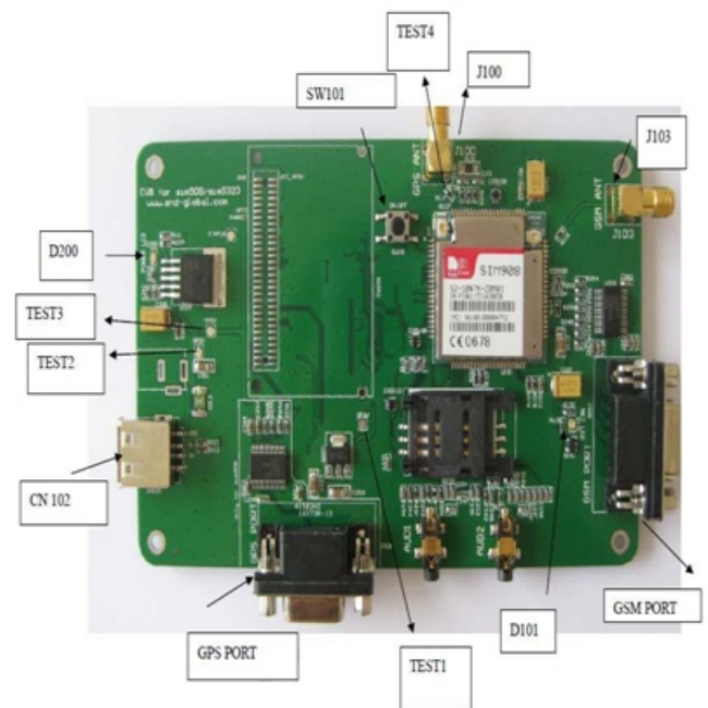
Figure 2 SIM908 GSM/GPS Module Board
