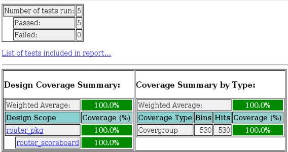
Figure 5: Functional Coverage of Router With Constrained Random Testcases
