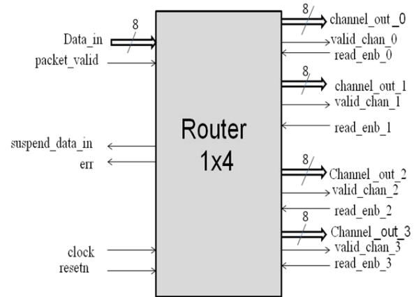
Figure1: Block Diagram of Router Protocol.
