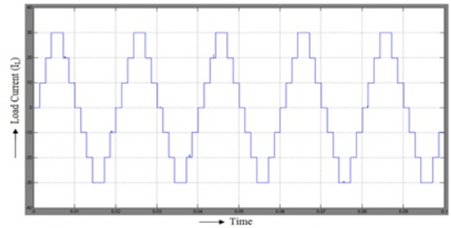
Fig 6.3 Seven levels of Inverter output current ( I_{inv} )
