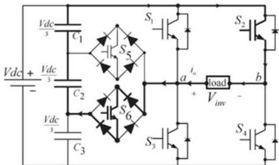
Fig 4.6 Inverter circuit for the output voltage (-2V_{dc}/3)
