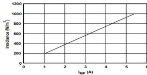
Figure 2.4 Irradiance vs IMP for 200 to 1000 W/m 2 .
