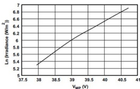
Figure 2.3 Irradiance vs VMP for 200 to 1000 W/m 2
