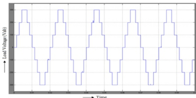
Fig 6.2 Seven levels of Inverter output voltage ( V_{inv} )
