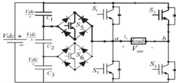
Fig 4.5 Inverter circuit for the output voltage (-V_{dc}/3)
