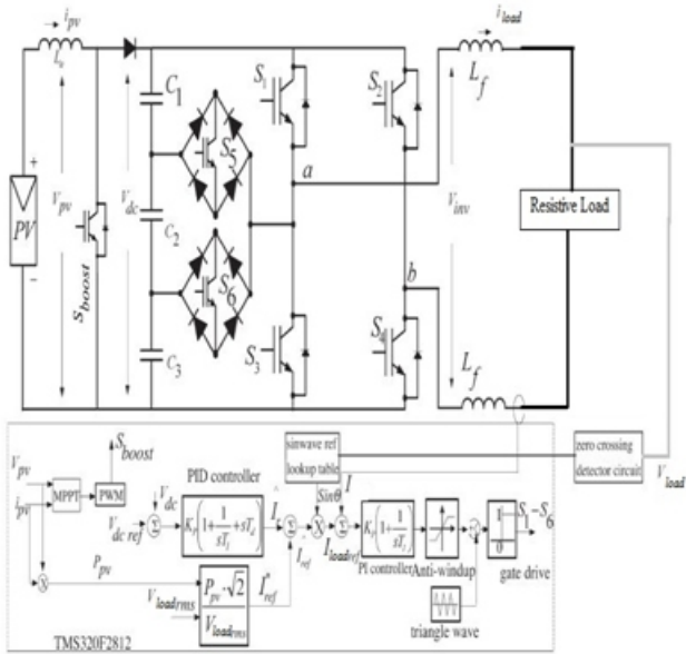
Fig. 5.1 Seven-level inverter with closed-loop control algorithm
