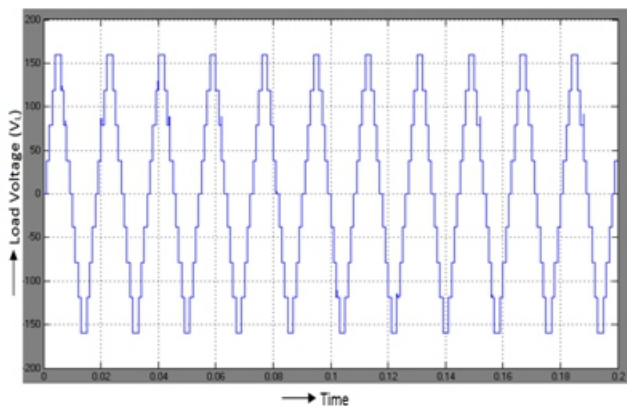
Fig 6.7 Nine levels of Inverter output voltage ( V_{inv} )
