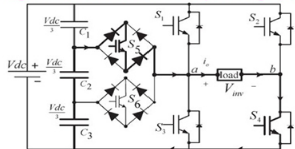
Fig 4.2 Inverter circuit for the output voltage ( 2V_{dc}/3 )
