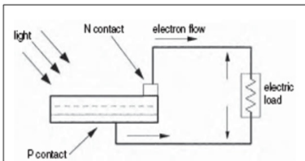
Fig 2.1: PV effect converts the photon energy into voltage across the p-n junction
