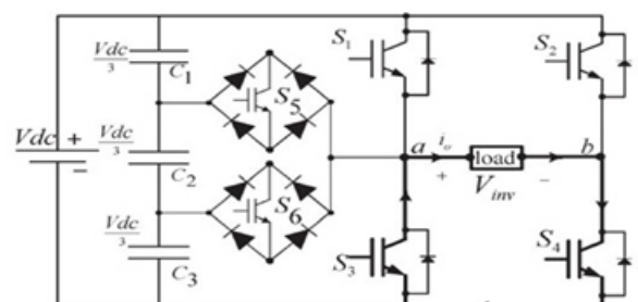
Fig 4.4 Inverter circuit for the output voltage (zero o)
