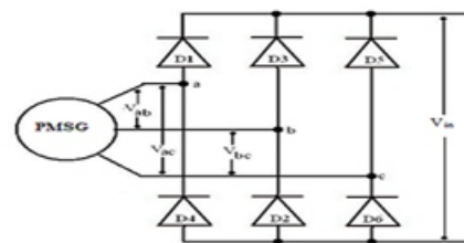
Fig.3. Three phase diode bridge rectifier
