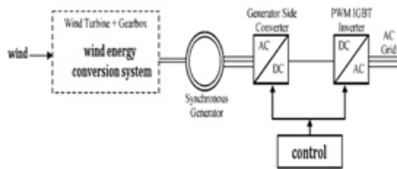
Fig. 1. Proposed Wind Energy Conversion System
