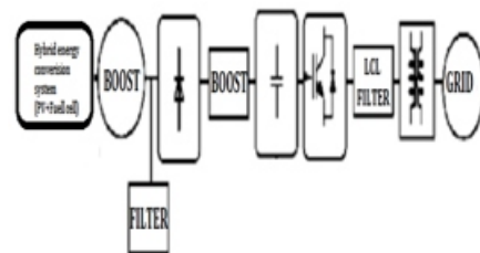
Fig.6. Hybrid energy conversion system connected to grid
