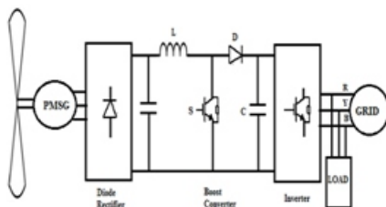
Fig.2. Block diagram of the system.
