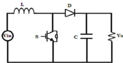
Fig.4. Basic schematic diagram of boost converter
