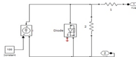
Fig.15. Simulink design for photovoltaic cell
