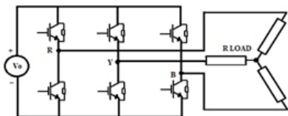
Fig.5. Three phase inverter
