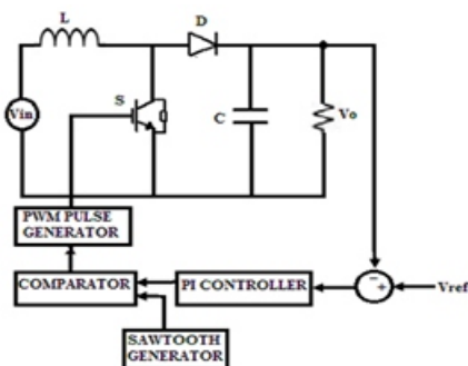
Fig.5. Closed loop boost converter
