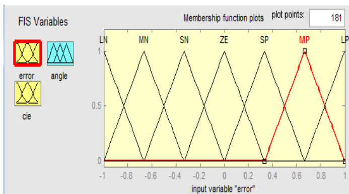
FIG (4): Input Membership Function of Fuzzy Logic Controller
