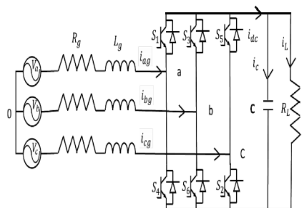
Fig.1 grid side VSC
