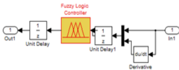
FIG(3): Structure of Control Mechanism for Grid Side Converter
