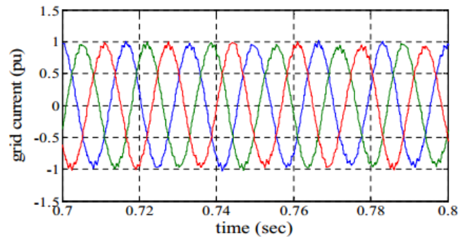
Fig (6) grid current
