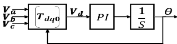
Fig.2 The configuration of three phase PLL
