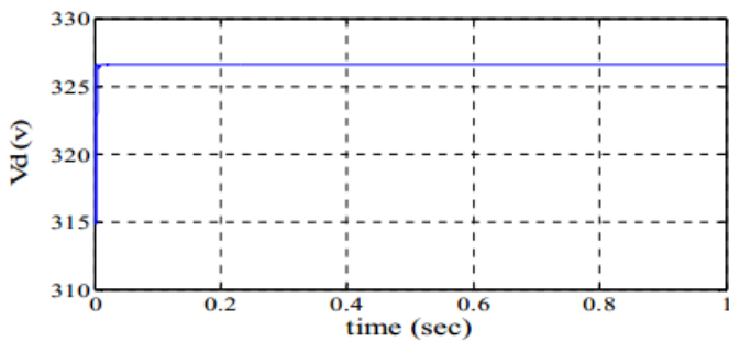
Fig (11) direct-axis voltage of grid
