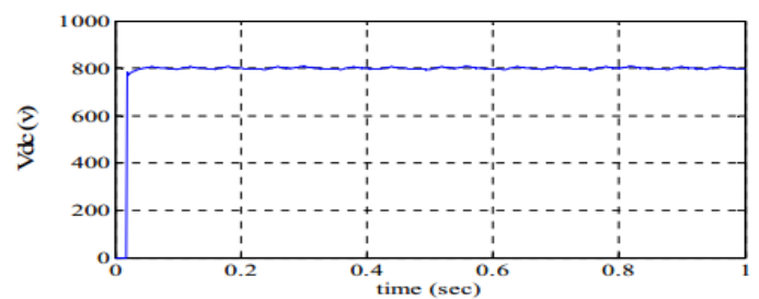
Fig (7) dc link voltage
