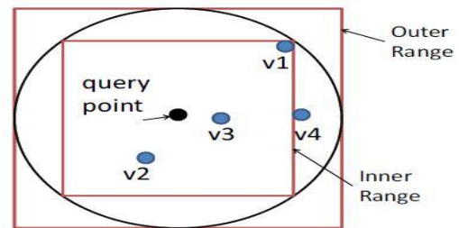
Fig. 2. Illustration for kNN-R Algorithm when k = 3.
