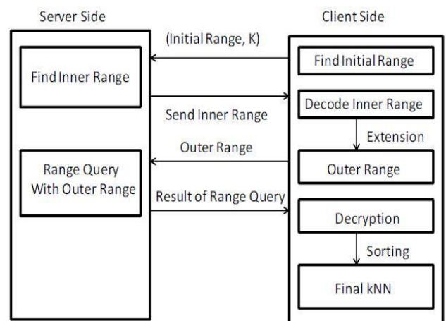
Fig. 3. Procedure of the KNN-R algorithm.
