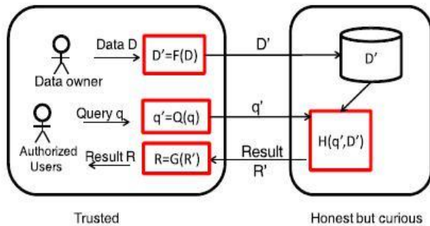
Fig. 1. The system architecture for RASP-based query services.
