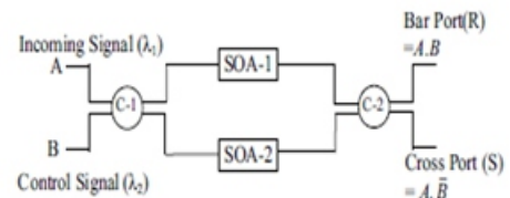
Fig. 1: Semiconductor Optical Amplifier based MZI Switch
