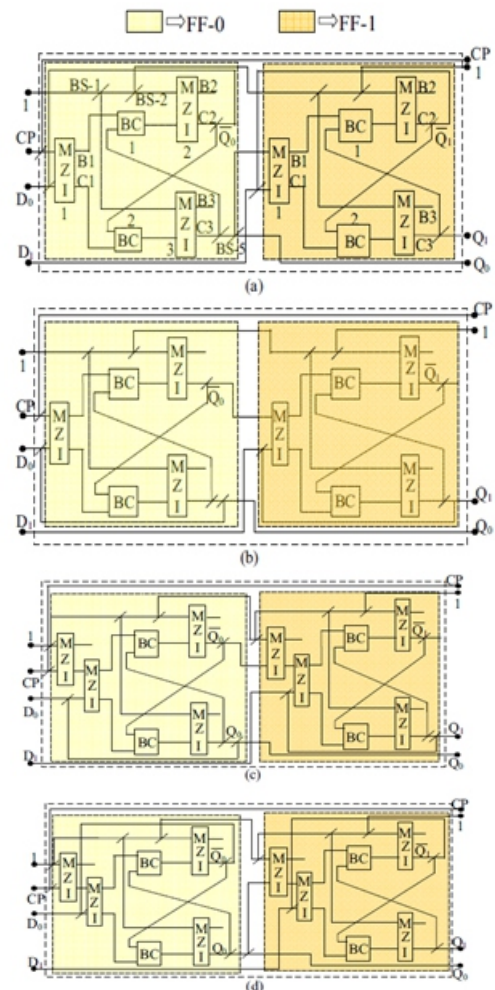
Fig. 3: Design of all optical reversible (a) asynchronous positive edge-triggered down counter, (b) asynchronous positive edge-triggered up counter (c) asynchronous negative edge-triggered down counter (d) asynchronous negative edge-triggered up counter using MZI switch. BC: Beam Combiner; BS: Beam Splitter; CP: Clock Pulse
