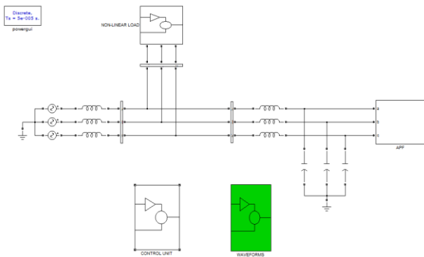
Fig.5 Simulation Circuit
