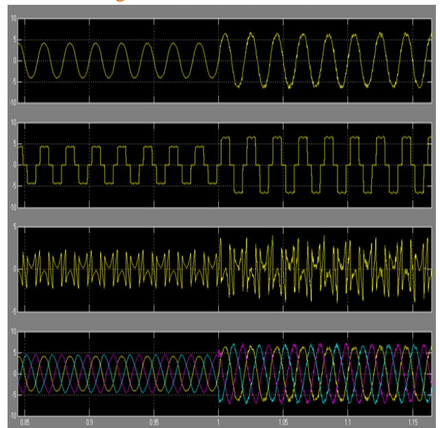
Fig.8 ISa,ILa,inv,ISabc(zoomed waveforms)
