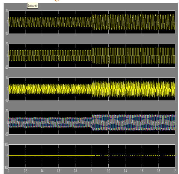
Fig.7 ISa,ILa,inv,ISabc,Vdc
