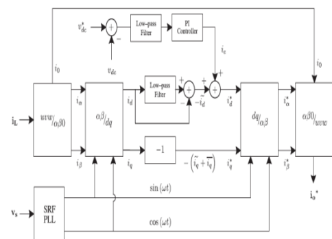
Figure 4: dq-based current reference generator block diagram .
