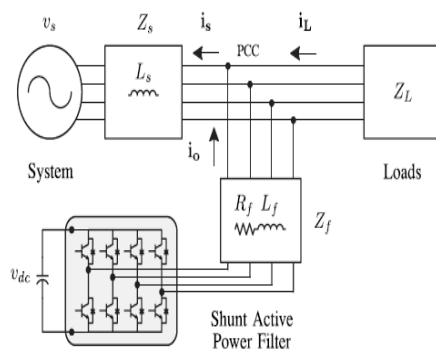
Fig. 2. Three-phase equivalent circuit of the proposed shunt active power filter.
