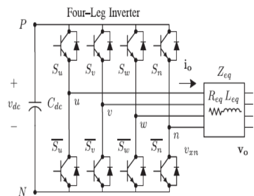
Fig. 3. Two-level four-leg PWM-VSI topology.
