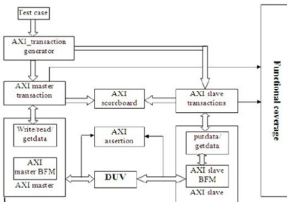
Figure 3 : AXI Verification Environment
