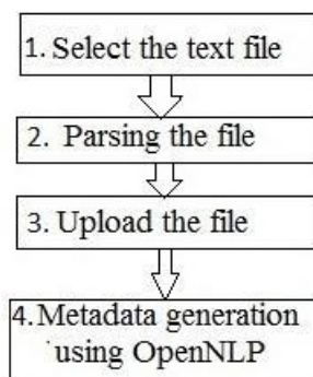
Fig 2: Information Extraction algorithm
