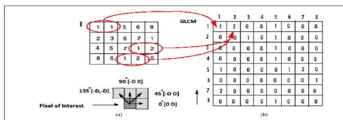
Figure.2 (a) GLCM directions and offset. (b) GLCM process using image
