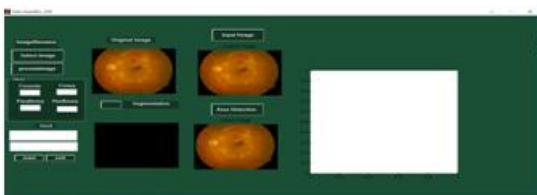
Figure.9 Segmentation
