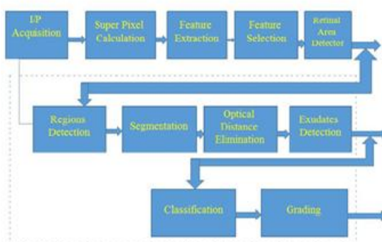
Fig.1 Proposed Method Block Diagram
