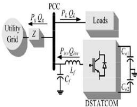
Fig. 1. Low voltage distribution grid under analysis with the voltage regulator
