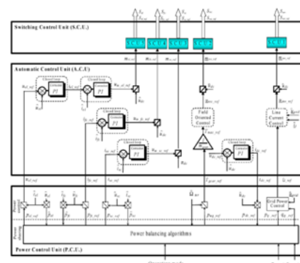
Fig. 7 Modelling and control of the HPS by the Energetic Macroscopic Representation.
