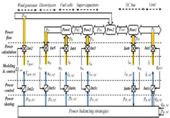
Fig. 8 Multilevel representation of the power modeling and control of the HPS.
