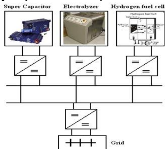
Fig. 3 Hybrid Power System Electrical Layout.
