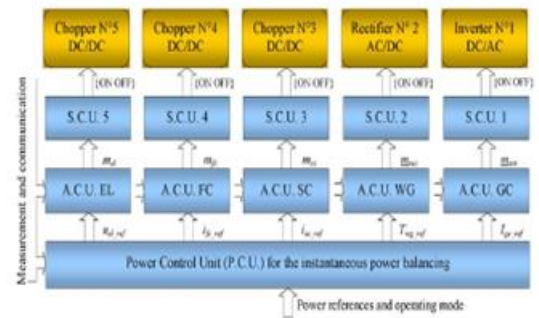
Fig. 6 Hierarchical control structure of the HPS]
