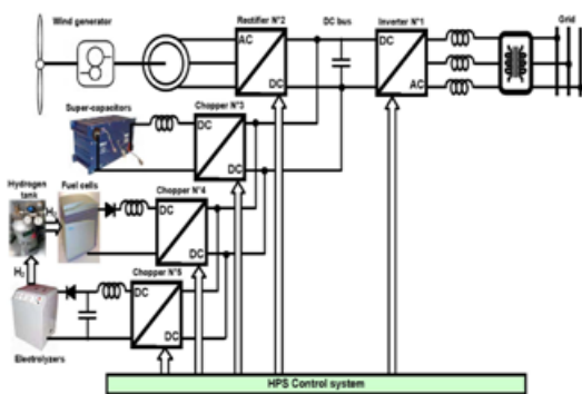
Fig.2. Structure of the studied wind/hydrogen/SC HPS.
