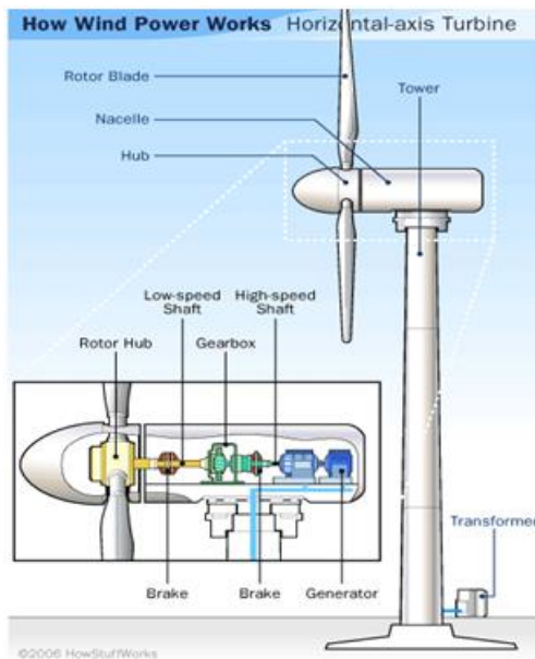
Fig. 1 Horizontal axis Turbine
