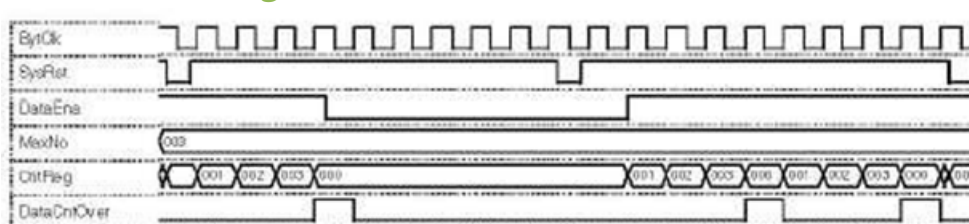
Fig. 6.1b: Simulation Indicate that, when the no of data is equal to the maximum number, then Data Cnt Over signal goes high
