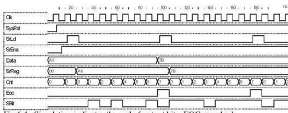
Fig 6.1d: Simulation Indicates that the end of constant bits. EOC goes high
