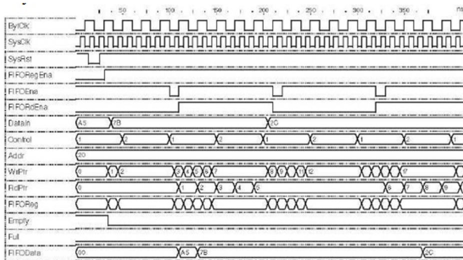
Fig 6.1a: Simulatio indicates enabling of FIFO on the raising edge of two clocks SysClk and ByteClk
