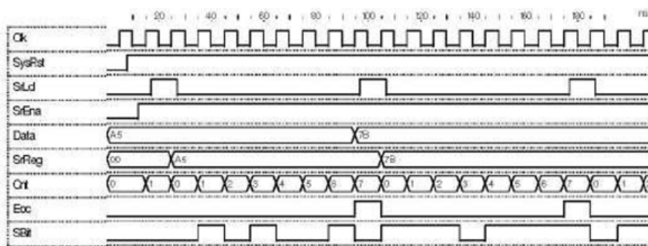
Fig 6.1c Simulation indicates the end of output bits, EOC goes high
