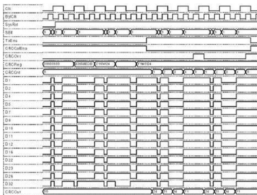
Fig 6.1e: Simulation indicate,at the end of transmission of data,CRC Over goes high
