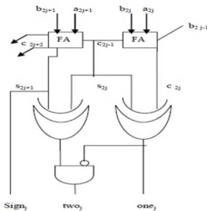
Fig. 3 Circuit diagram for proposed MBRS
