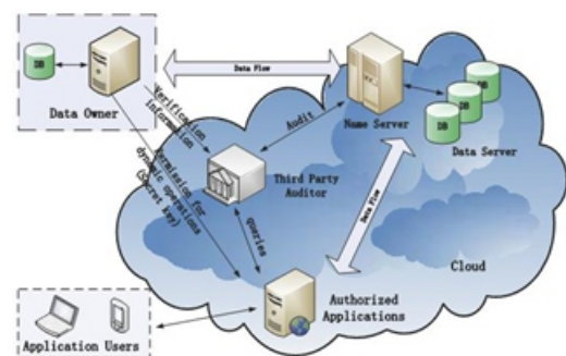
Figure1 : Architecture Diagram
