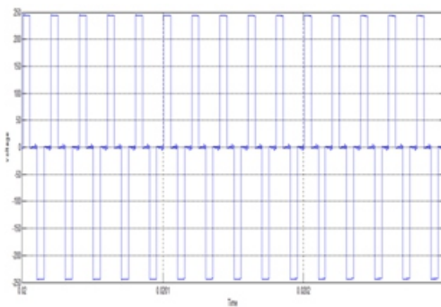
Fig.10. Simulated output wave form of the voltage at primary winding of the transformer of the proposed converter.
