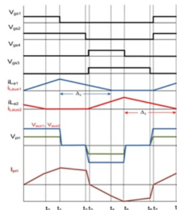
Fig.3 Typical waveforms describing the modes of operation
