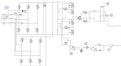
Fig.11. Matlab/Simulink Model of Proposed Converter Operated under Closed Loop Manner.
