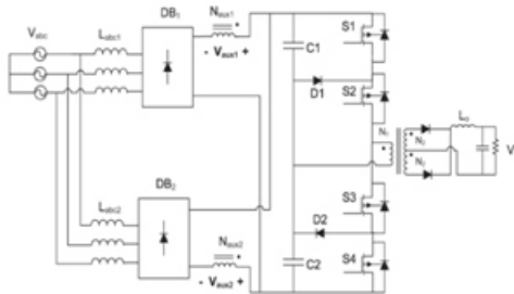
Fig.2 Proposed interleaved three-phase three-level converter
