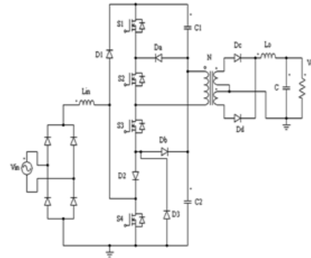
Fig.1 Three level single stage converter
