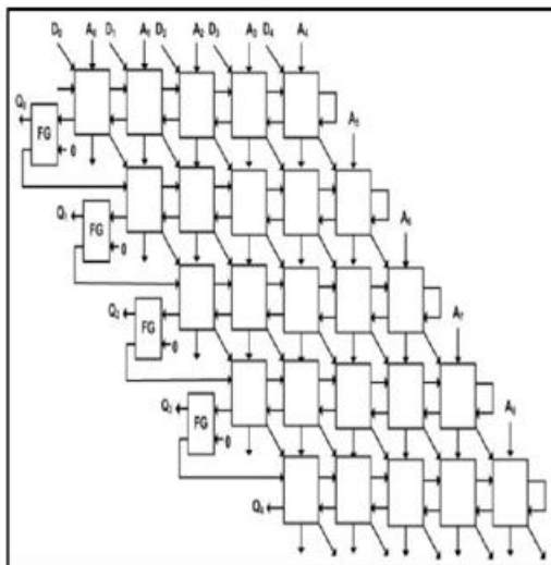
Figure.14. Proposed n-bit reversible division circuit
