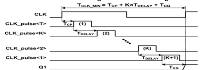
Fig. 7. Minimum clock cycle time of the proposed shift register.
