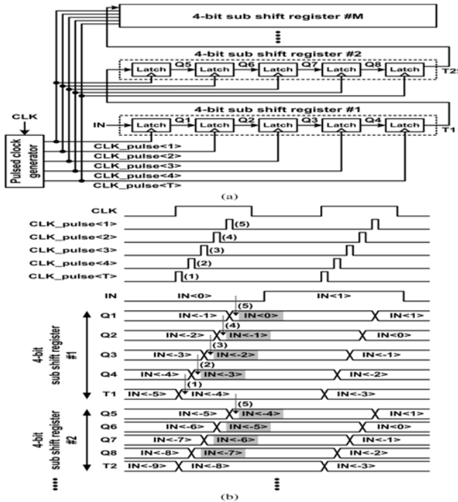
Fig. 5. Proposed shift register. (a) Schematic. (b) Waveforms.
