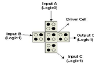
Fig.2 Majority Gate
