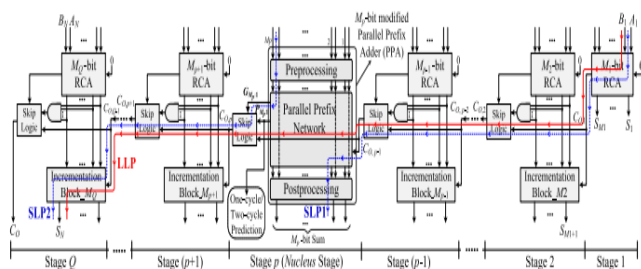
Fig. 6. Structure of the proposed hybrid variable latency CSKA.
