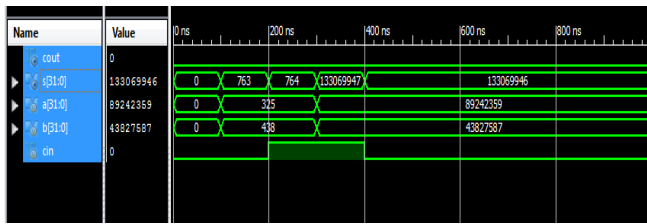
Figure 8-2: Simulated output for Variable Stage Size Carry Skip Adder
