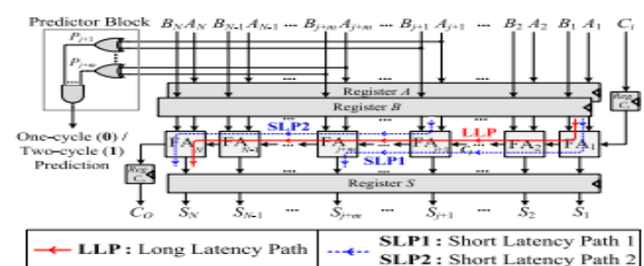
Fig. 5. Generic structure of variable latency adders based on RCA.
